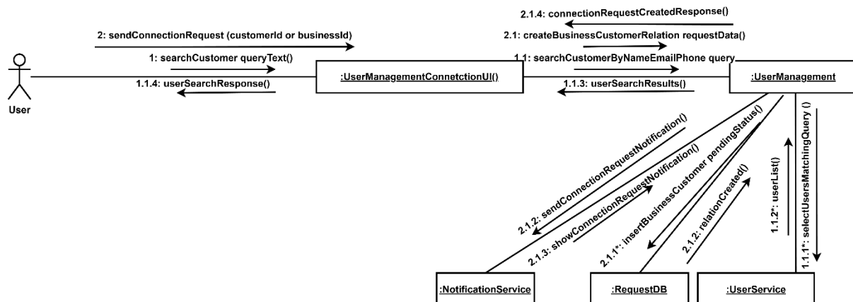
Figure 18: Collaboration Diagram – User Management
