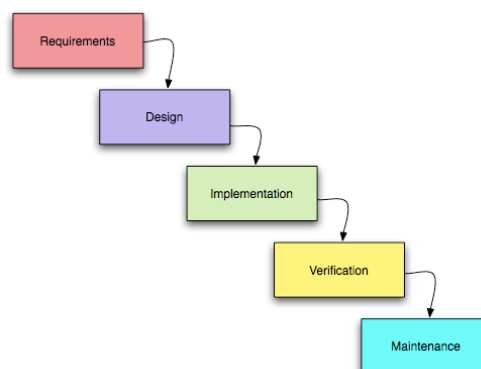
Figure 9: Waterfall model
