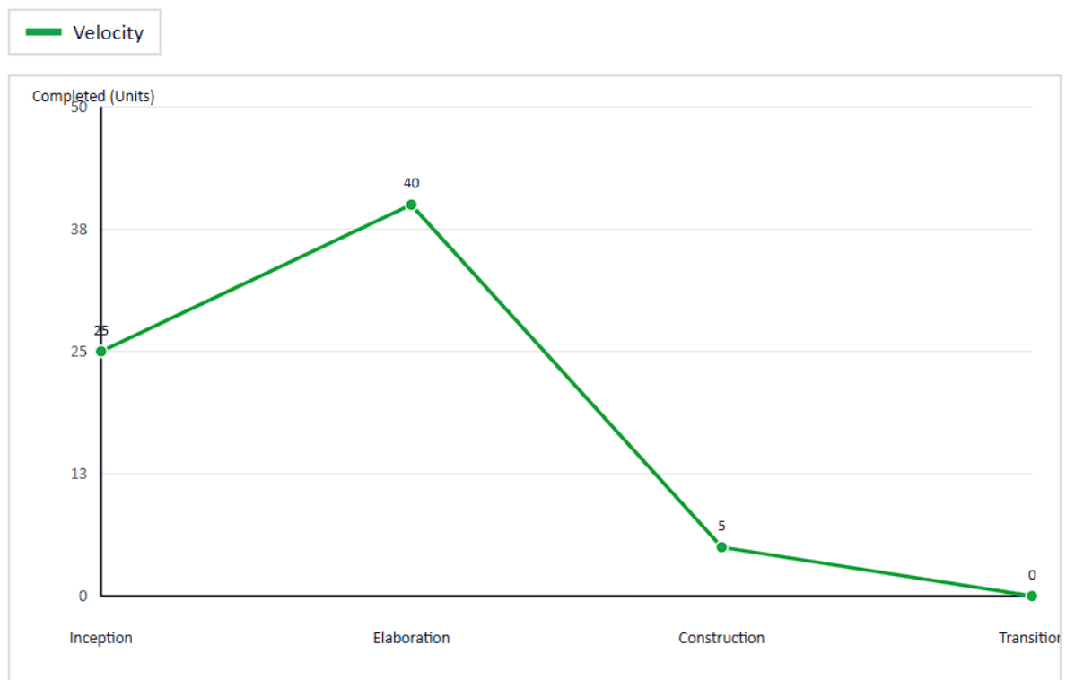
Figure 61: Velocity Chart
