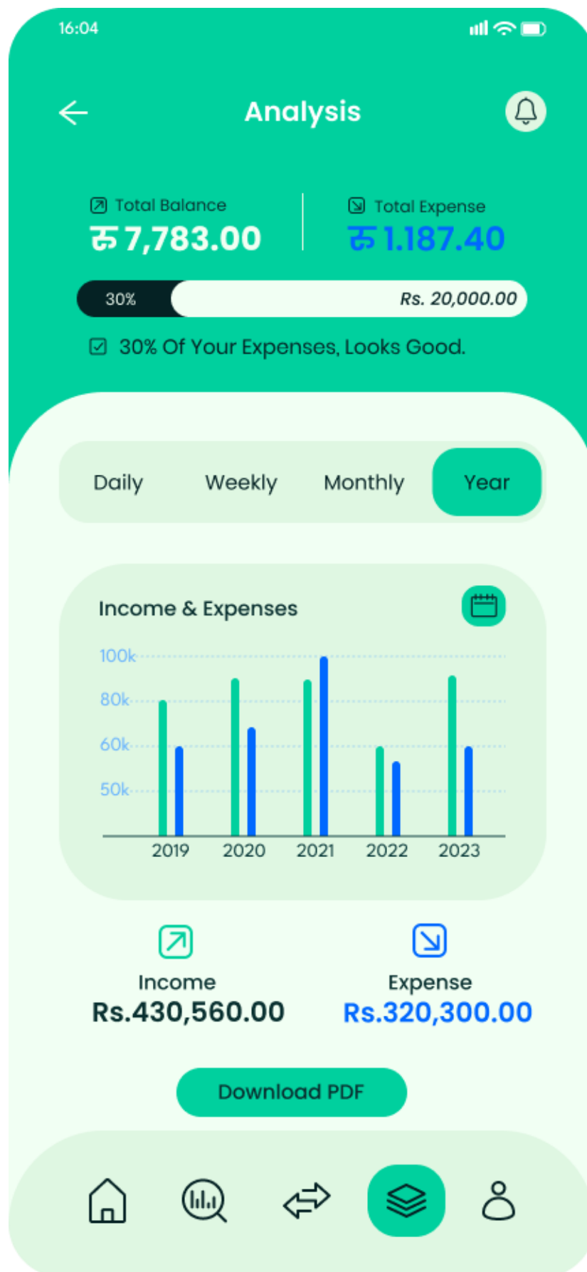
Figure 56: Analytics Screen
