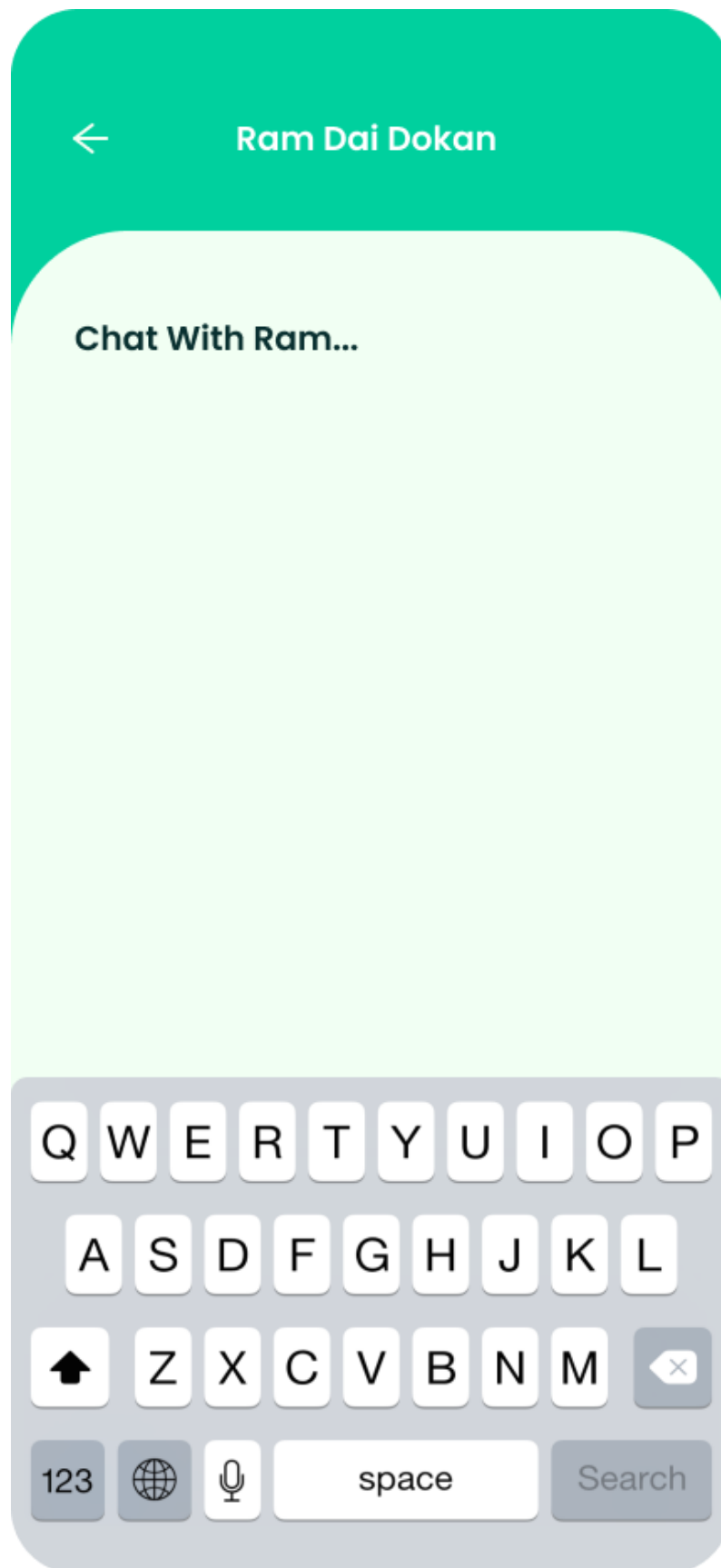
Figure 43: Chat Screen
