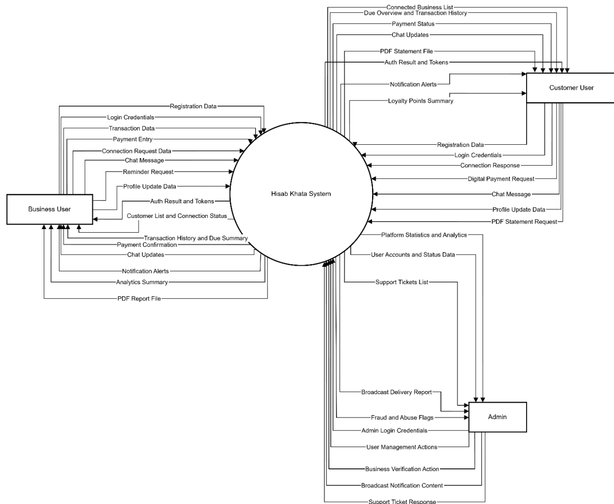
Figure 35: Dataflow Diagram
