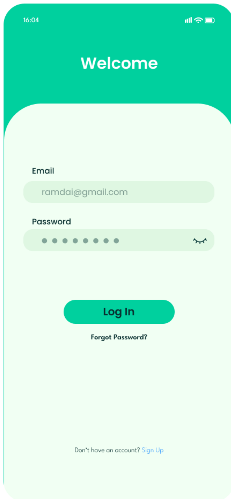
Figure 39: Login Screen
