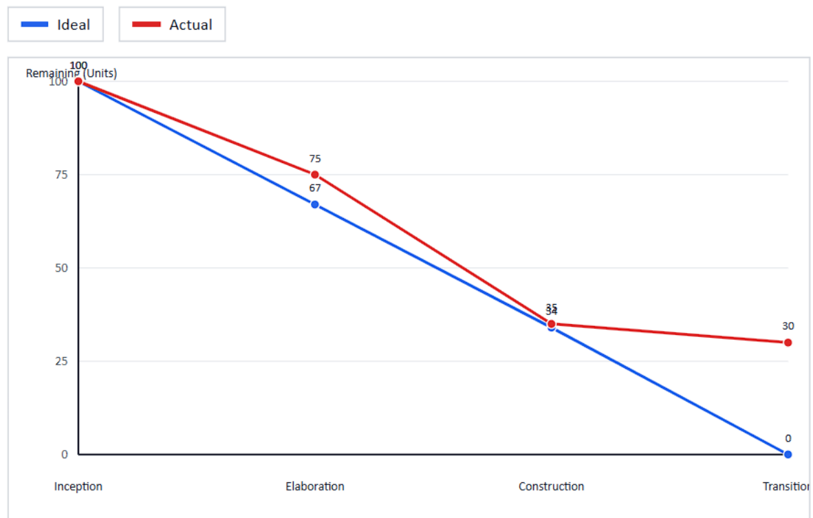
Figure 62: Burndown Chart
