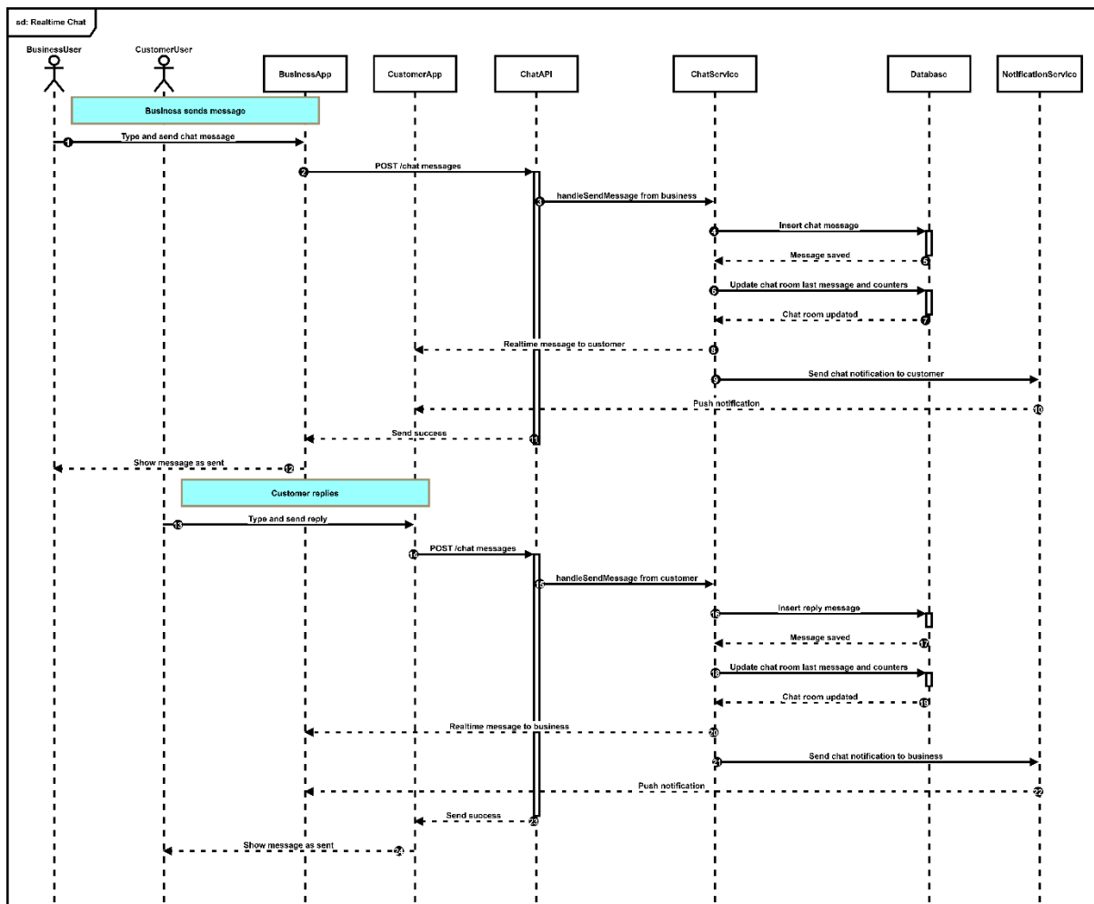
Figure 27: Sequence Diagram – Realtime Chat
