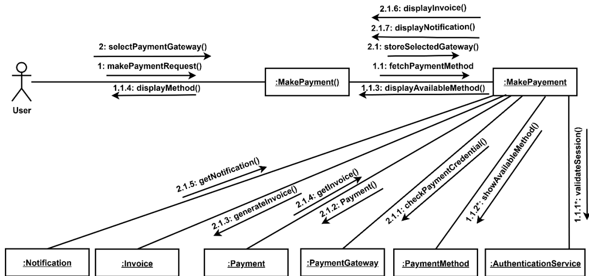
Figure 15: Collaboration Diagram – Make Payment
