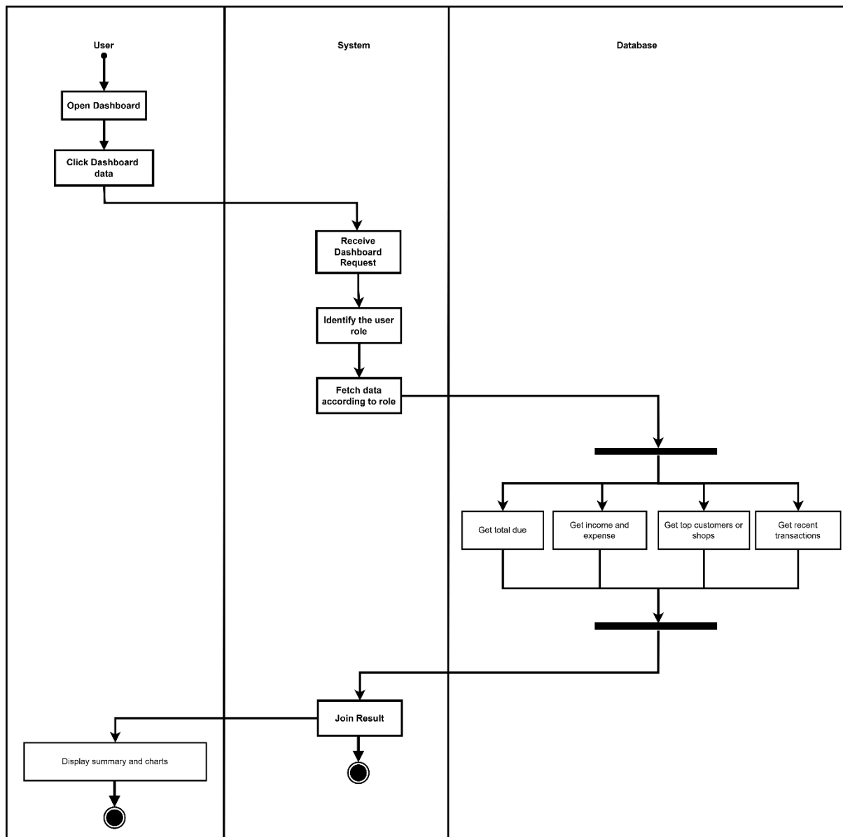
Figure 32: Activity Diagram – Dashboard and Analytics
