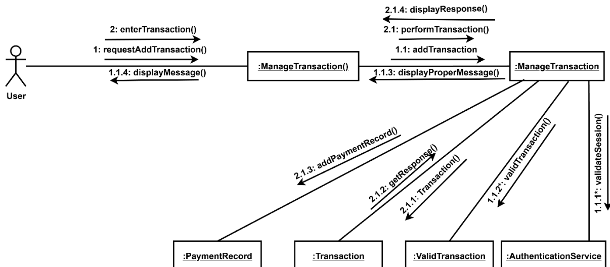
Figure 16: Collaboration Diagram – Manage Transaction
