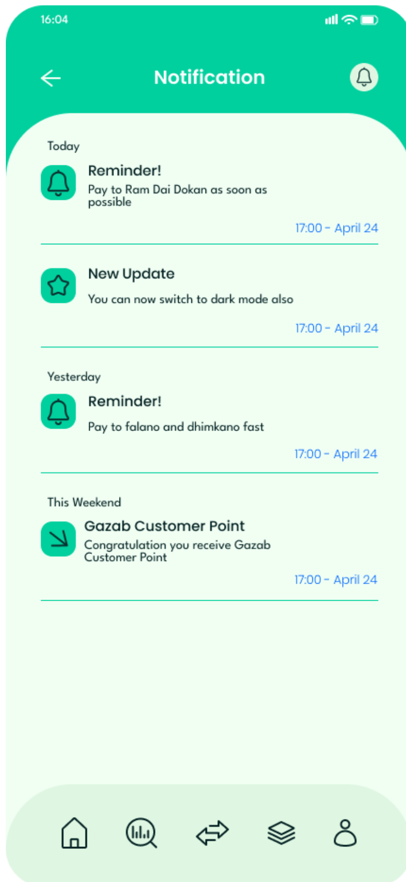
Figure 50: Notification Screen
