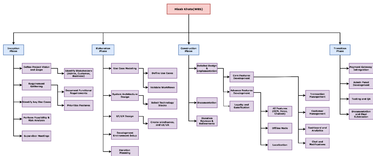
Figure 97: WBS Diagram
