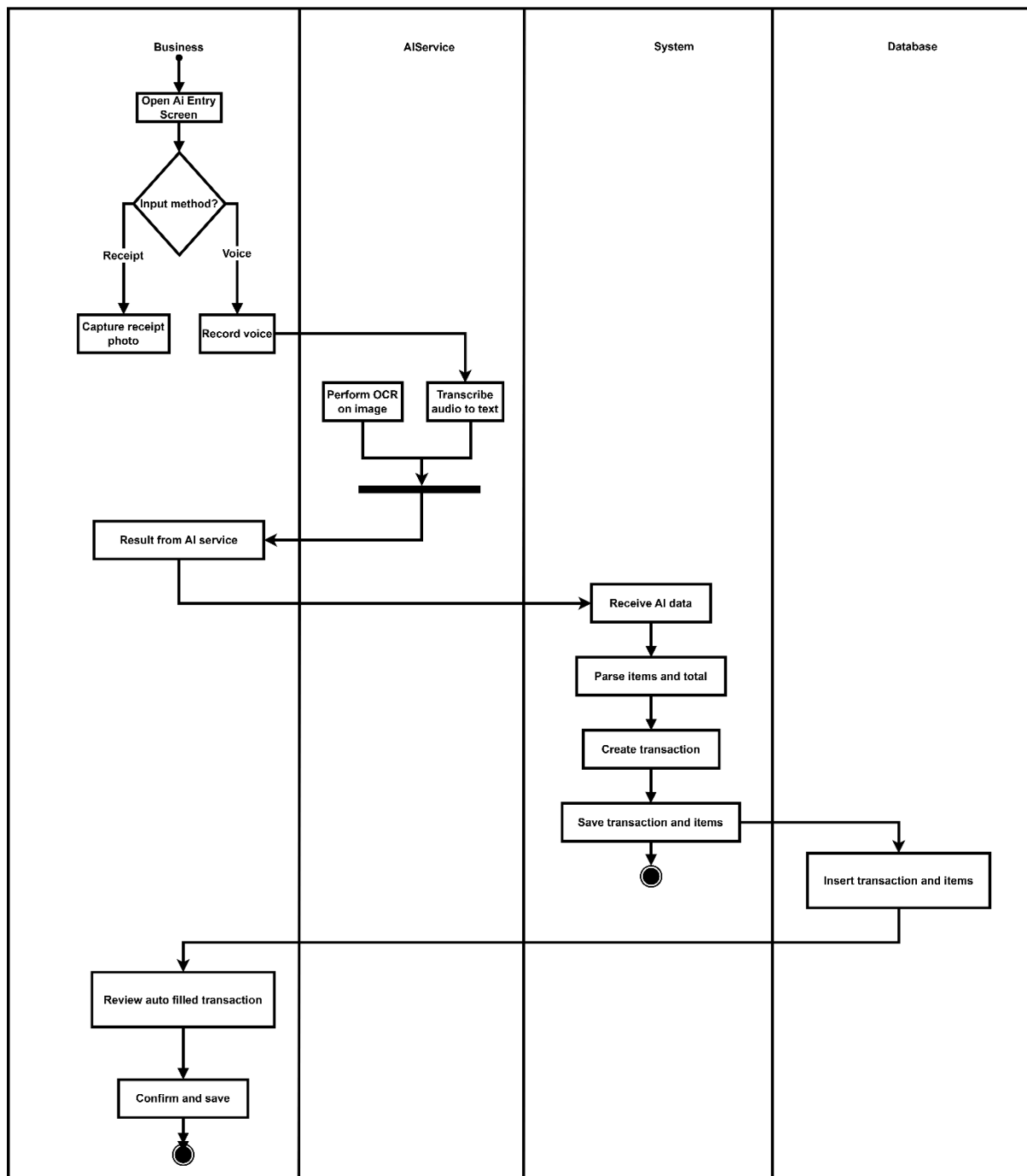
Figure 33: Activity Diagram – AI Features
