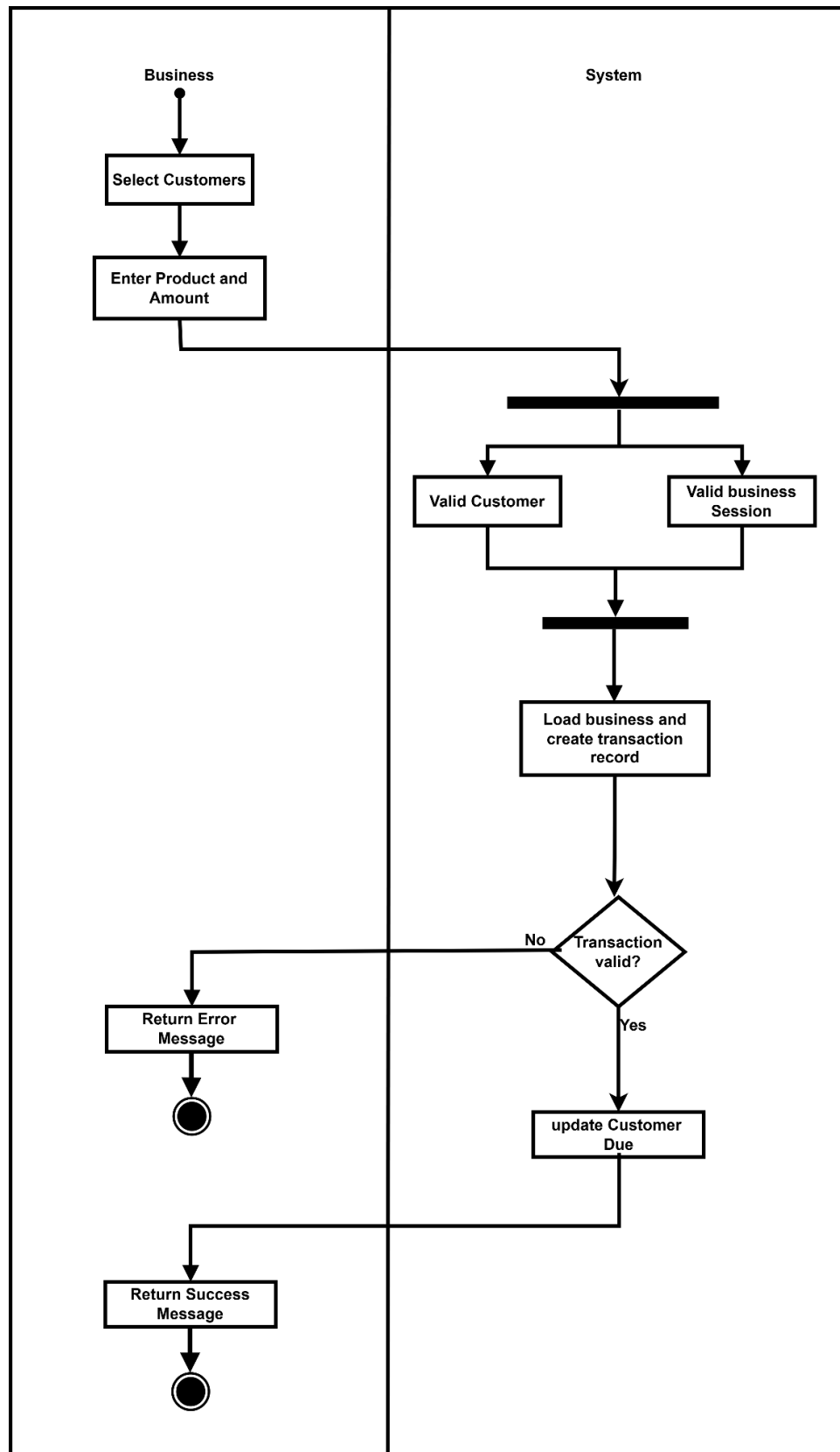
Figure 30: Activity Diagram – Transaction Management
