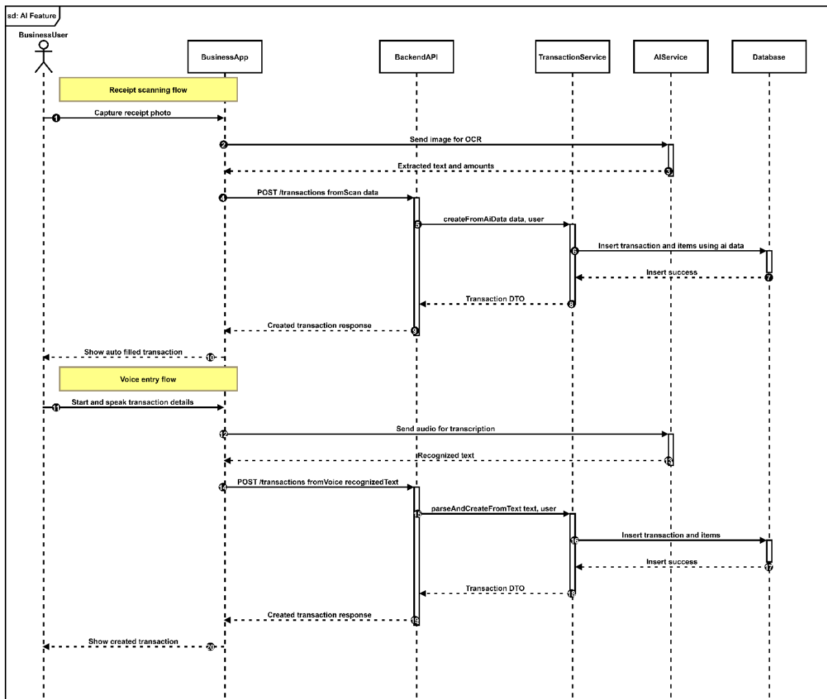
Figure 25: Sequence Diagram – AI Features
