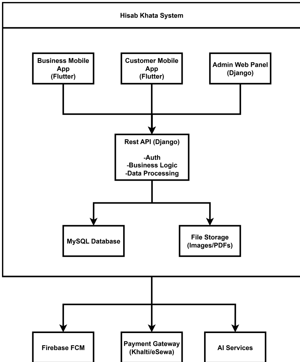
Figure 13: System Architecture/Context Diagram
