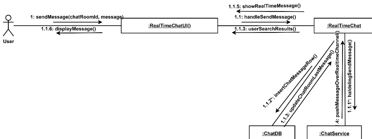
Figure 19: Collaboration Diagram – Realtime Chat
