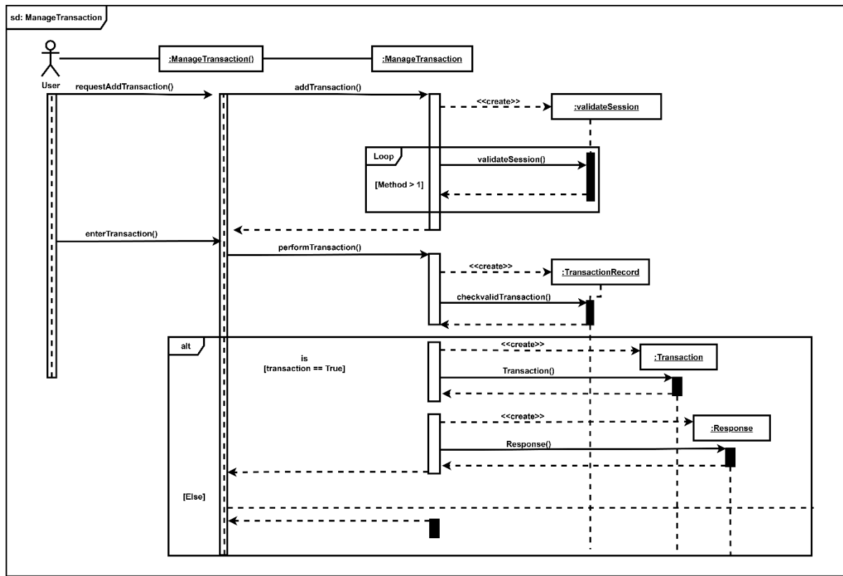
Figure 21: Sequence Diagram – Manage Transaction
