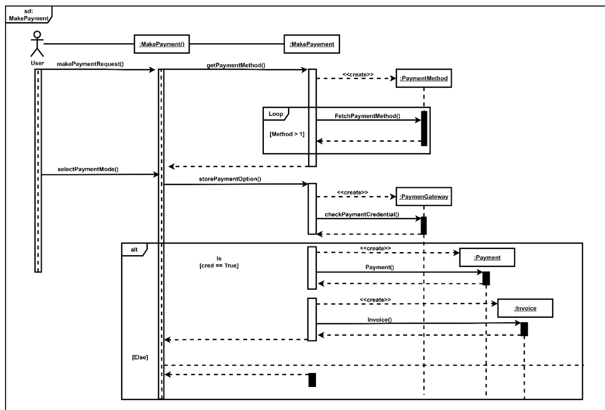
Figure 20: Sequence Diagram – Make Payment
