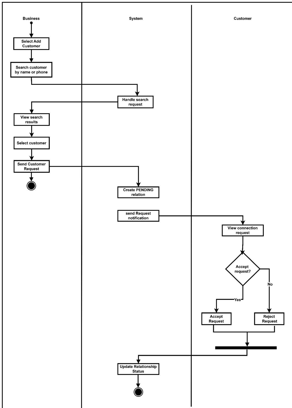
Figure 31: Activity Diagram – Customer Management
