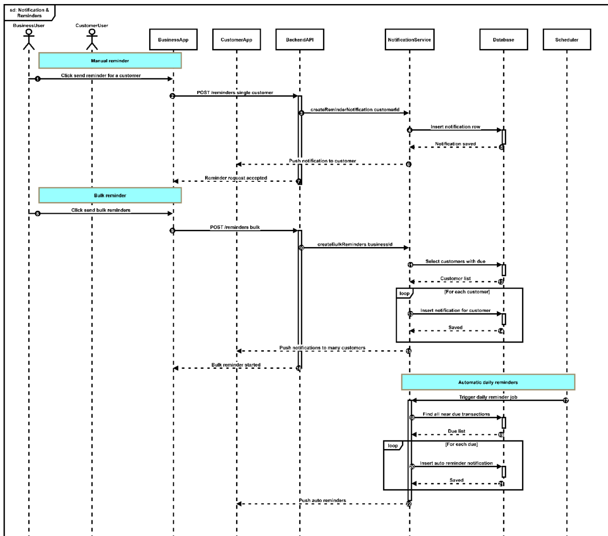
Figure 26: Sequence Diagram – Notification and Reminders
