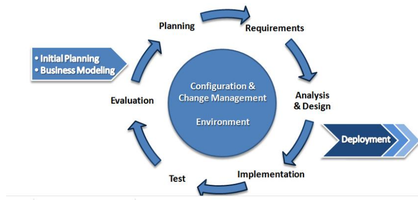
Figure 12: Process of RUP Methodology
