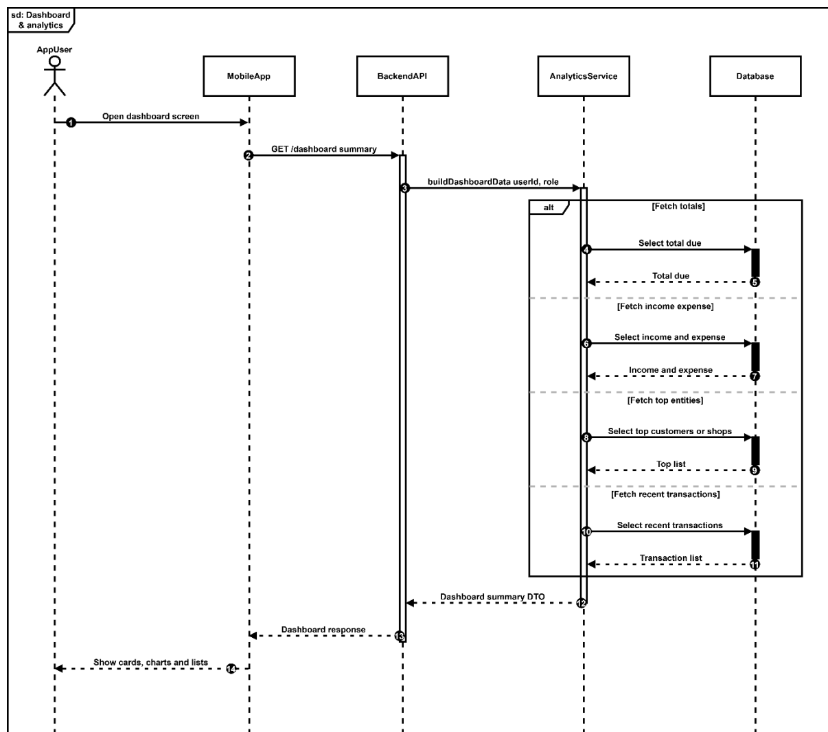
Figure 23: Sequence Diagram – Dashboard and Analytics
