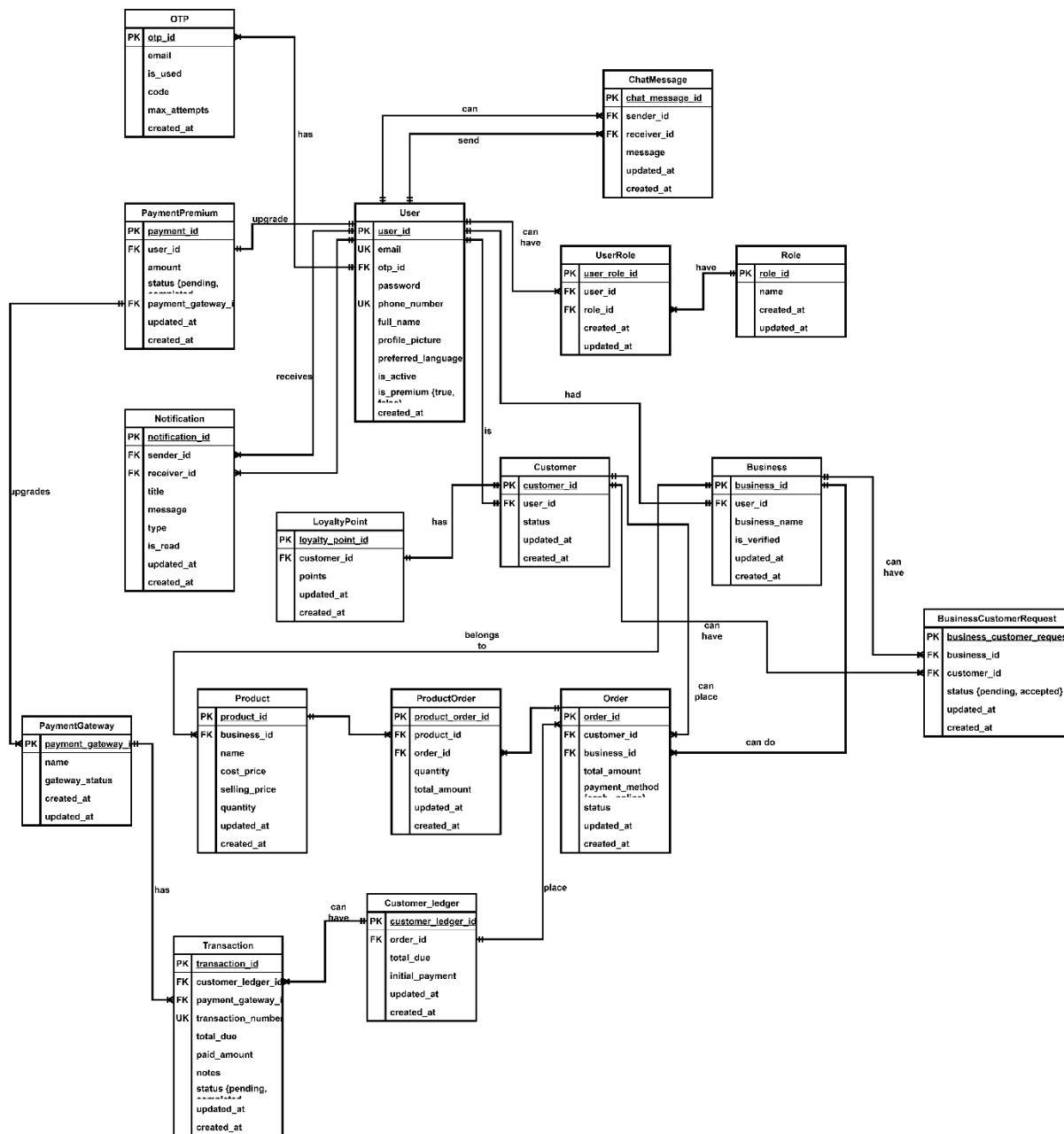
Figure 14: Entity Relationship Diagram
